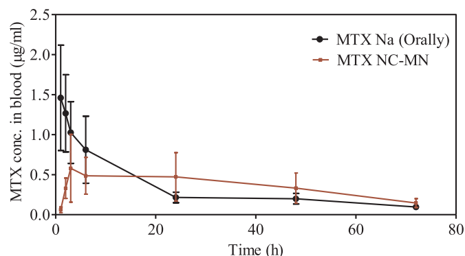
Fig. 6. MTX pharmacokinetic profiles in blood after administrating MTX Na solution by oral gavage and MTX NC-MN application to healthy female Sprague Dawley rats. Data is reported as means \pm S.D., ( n = 5 ).
